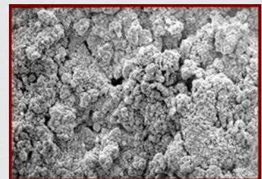
New Lead Sponge Battery Plate
