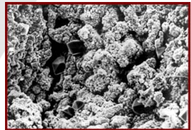
Final Recovery of the Active Sponge Lead
